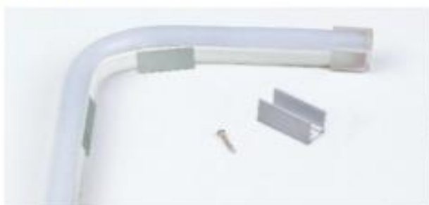
90° Installation
